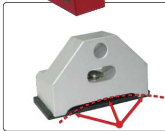
▲ Hybrid clamp has a sheathed high tensile leaf spring. Distributes load evenly to prevent crown collapsing.
