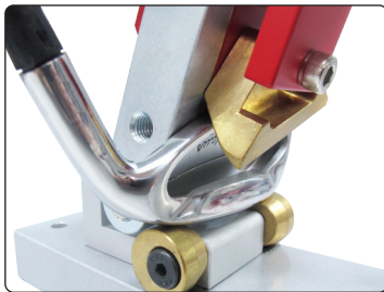
▲ Offset and indexable conical sheaves adapt to sole width and bounce angle of irons
