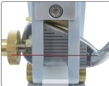
▲ Clear sighting of grooves ensures clubhead is set at the correct lie angle.
