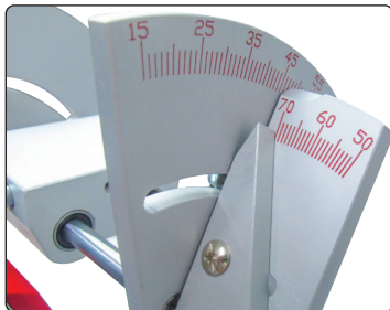
▲ Precision machined and engraved lie and loft protractor accurate 0.5°
