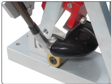
▲ Self-aligning pads adapt to sole radius of hybrids. Padded top clamp complies with crown curvature.
