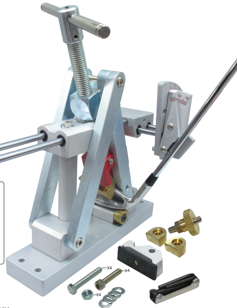
▲ Non-marring clamps, sheaves and pads included.
