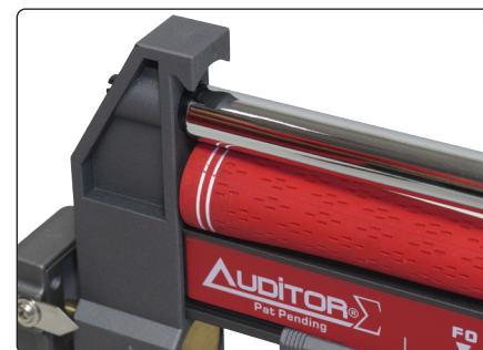
▲ Swing weighing grippless clubs with the built in grip cap compensator
