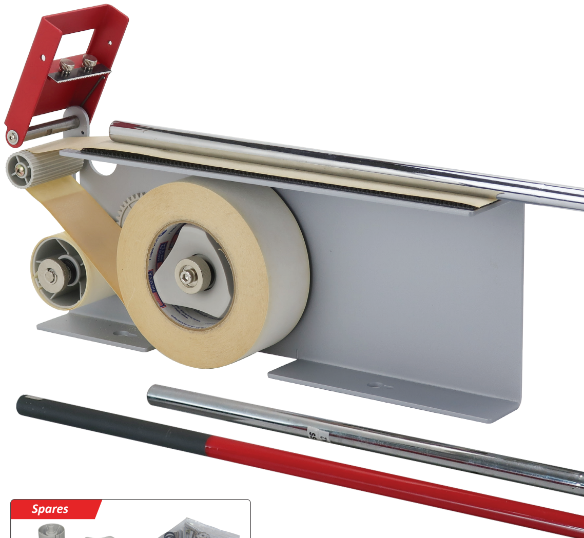
▲ Tape is pulled out and rested on the non-stick rolling platform.
