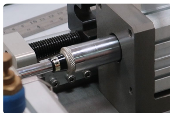
▲ Micrometric ferrule installer & press provide power and precision in a compact package.
