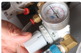
▲ Regulated air pressure for adjusting the pneumatic vise clamping force.
