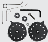
1102xx-SK3 Metered Gear set kit
