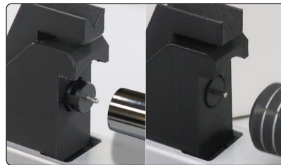
▲ Pre-assembled grippless clubs can also be swingweighted before final assembly.
